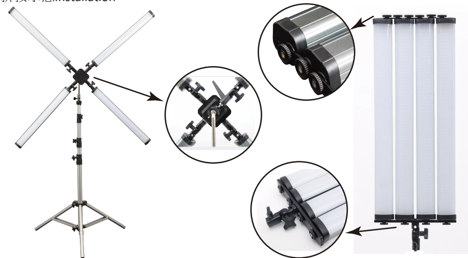
●SPR-200B-4棒灯连接配件拼接示意 SA1 with SPR-200B-4 X-Bracket
