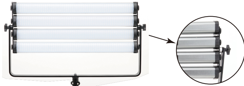
●SA1-U棒灯U架拼接示意 SA-1 With U-Bracket
